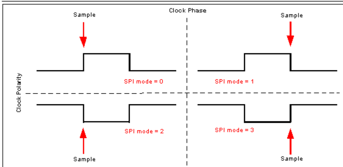
Figure 19.4: SPI modes selectable on SPI
